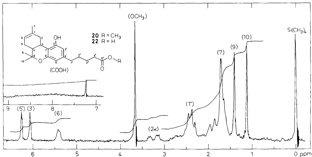
Fig. 1. 90-MHz- ^1\text{H} -NMR. spectra of methyl \Delta^1(6) -THC-5''-oate ( 20 ) and \Delta^1(6) -THC-5''-oic acid ( 22 ) in \text{CDCl}_3 . Peak at \delta = 3.7 ppm only in 20 , peak at \delta = 7.5\text{--}8.5 ppm only in 22 .
