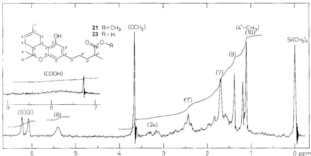
Fig. 2. 90-MHz- ^1\text{H} -NMR. spectra of methyl 4''(R,S)-methyl- \Delta^1(6) -THC-5''-oate ( 21 ) and 4''(R,S)-methyl- \Delta^1(6) -THC-5''-oic acid ( 23 ) in \text{CDCl}_3 . Peak at \delta = 3.7 ppm only in 21 , peak at \delta = 7.5 – 8.5 ppm only in 23 .
